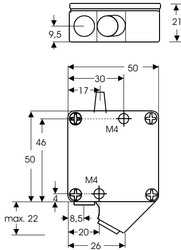
Sensor head Type / 0,5 weight 250 g, cable length 2 m
