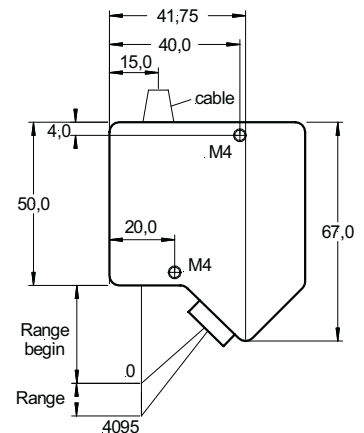
Sensor head Type / 2 / 4 / 10 / 20 weight 240 g, cable length 2 m
