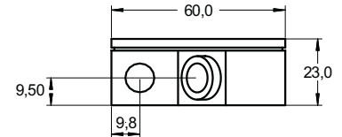
Sensor head M27L / 1,5 weight 290 g, cable length 2 m
